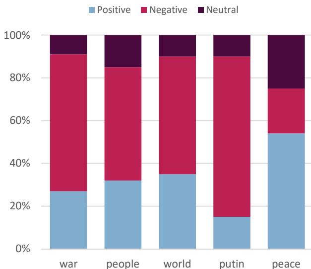
Fig. 4. Category Wise Sentiment Analysis of the Top Five Words.
