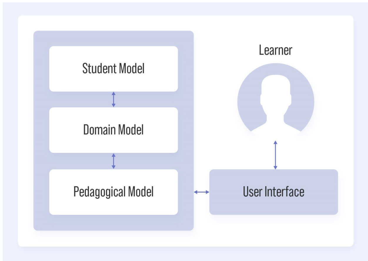
Figure 1. Generic Intelligent Tutoring System Architecture
