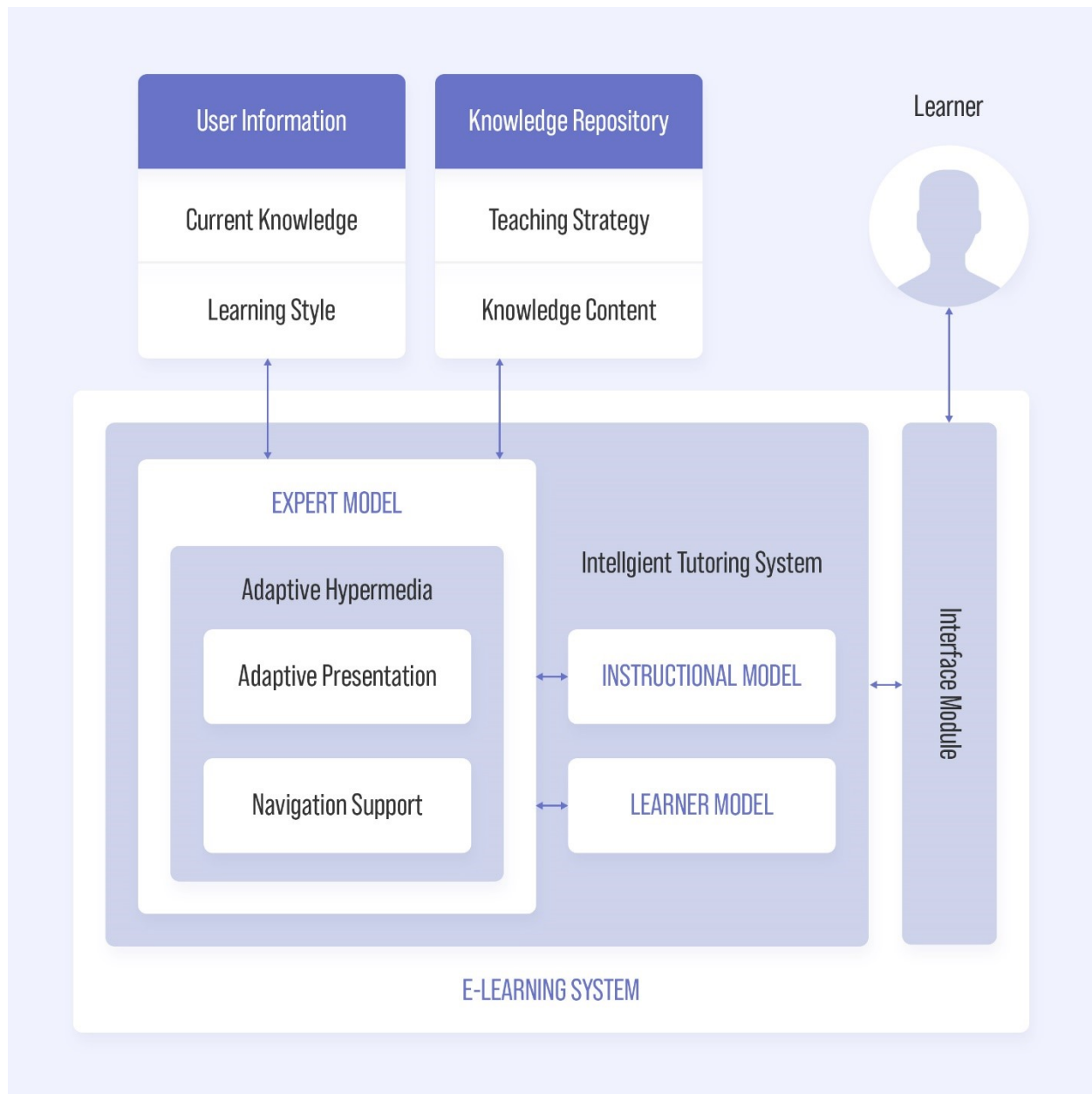
Figure 3. E-Learning with Intelligent Tutoring System
